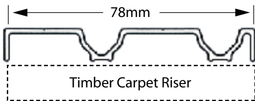
SILL TRACK
